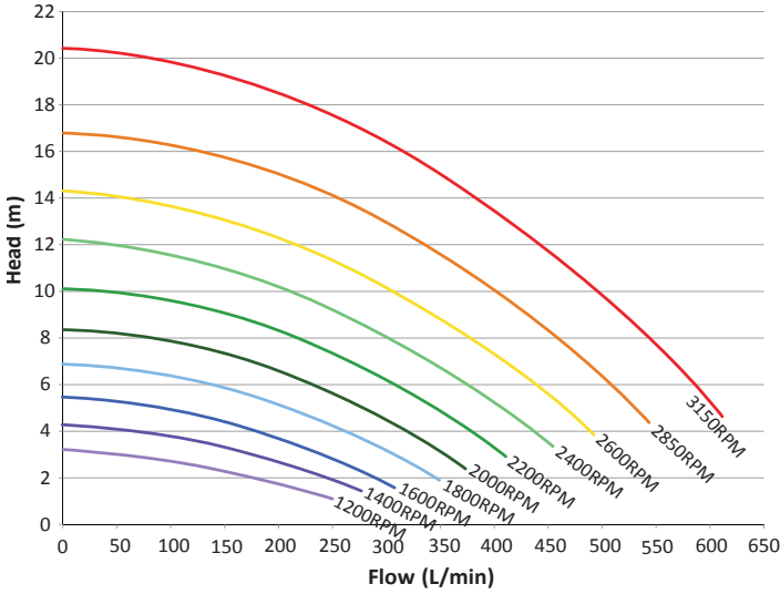
EnviroMAX 1500 Performance Chart
